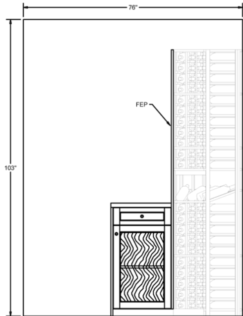
ELEVATION -A-
